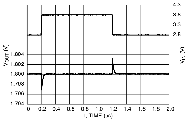
Figure 49. Line Transients, 1.8 V Version, t_{\text{R}} = t_{\text{F}} = 5 \mu\text{s} , I_{\text{OUT}} = 30 \text{ mA} , \text{AE} = V_{\text{IN}} \text{ V}
