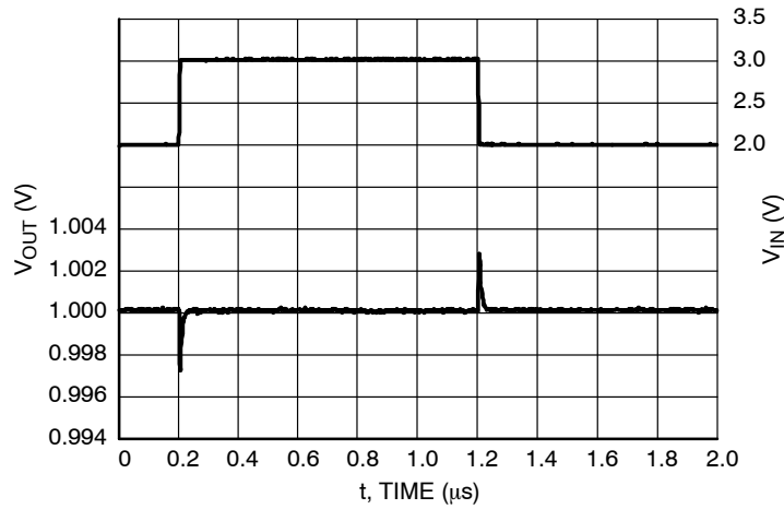
Figure 47. Line Transients, 1.0 V Version, t_{\text{R}} = t_{\text{F}} = 5 \mu\text{s} , I_{\text{OUT}} = 30 \text{ mA} , \text{AE} = V_{\text{IN}} \text{ V}
