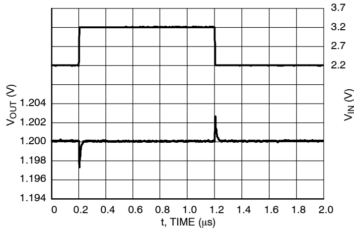
Figure 48. Line Transients, 1.2 V Version, t_{\text{R}} = t_{\text{F}} = 5 \mu\text{s} , I_{\text{OUT}} = 30 \text{ mA} , \text{AE} = V_{\text{IN}} \text{ V}
